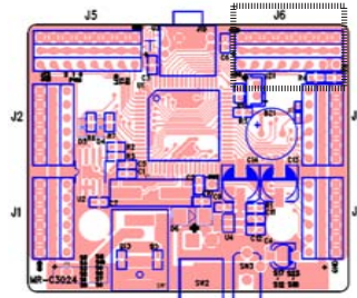
Robonova Controller Board
